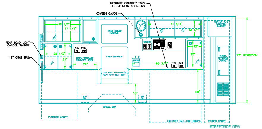
STREETSIDE VIEW
