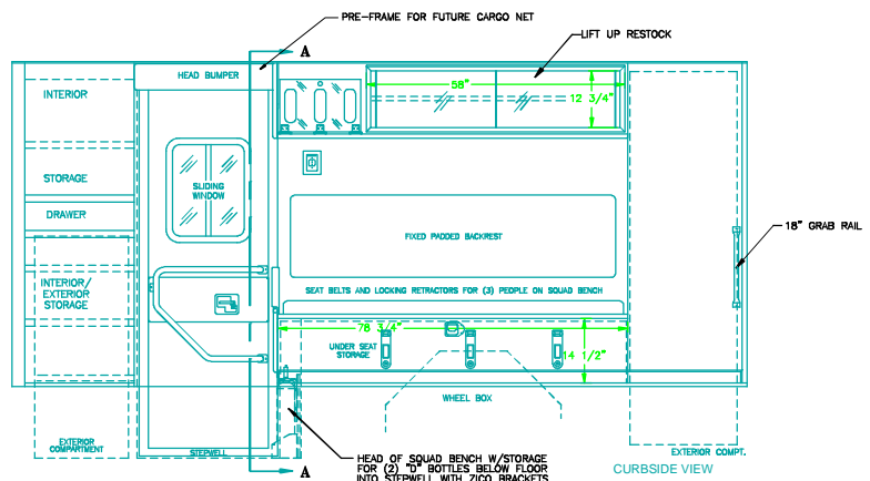
CURBSIDE VIEW
