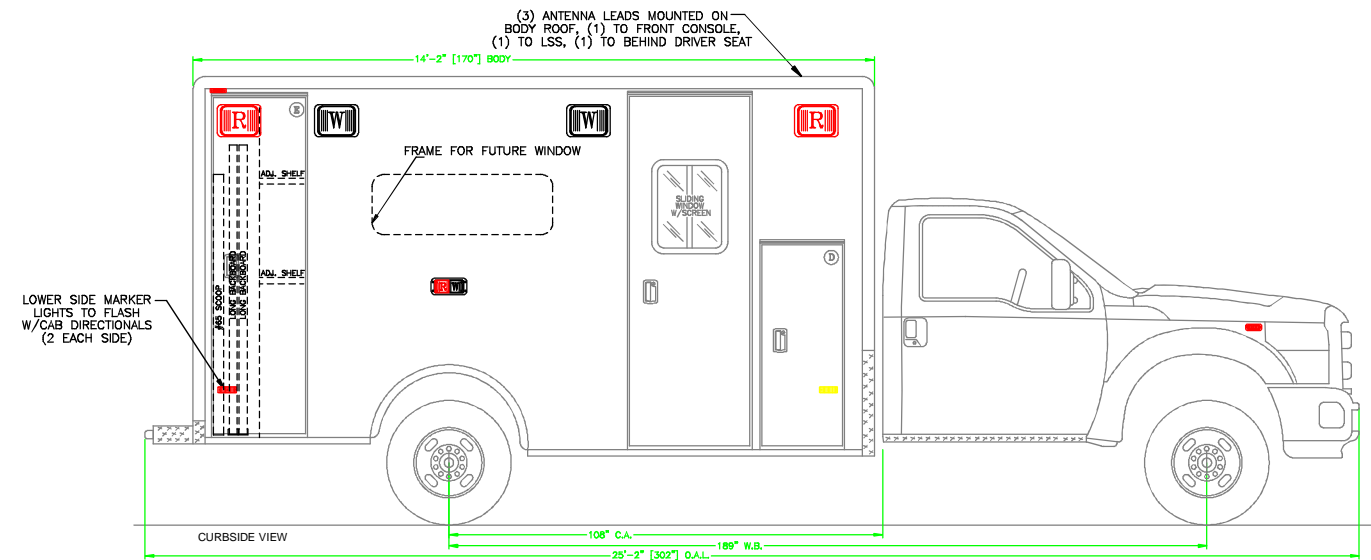
CURBSIDE VIEW
