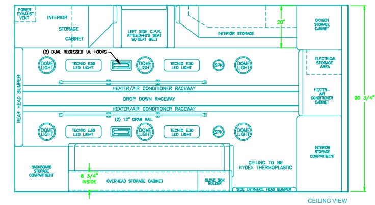
CEILING VIEW
