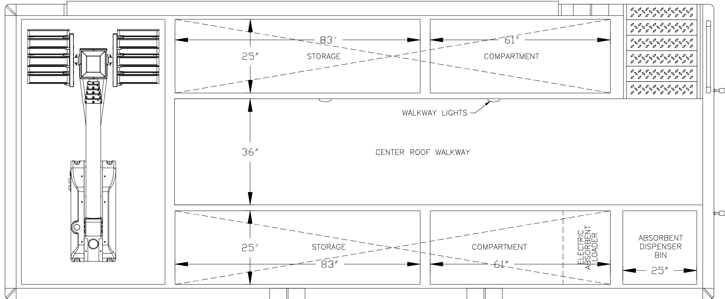
ROOF VIEW
